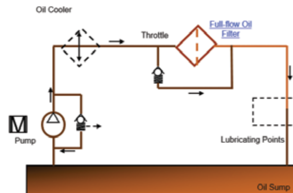
Bypass Circuit Diagram
