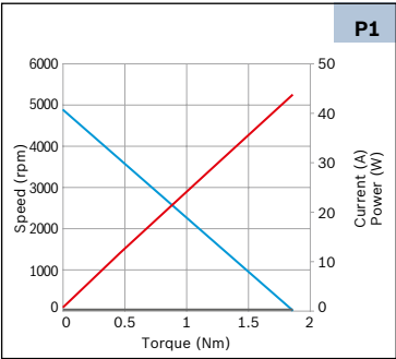
Performance curve (P)
