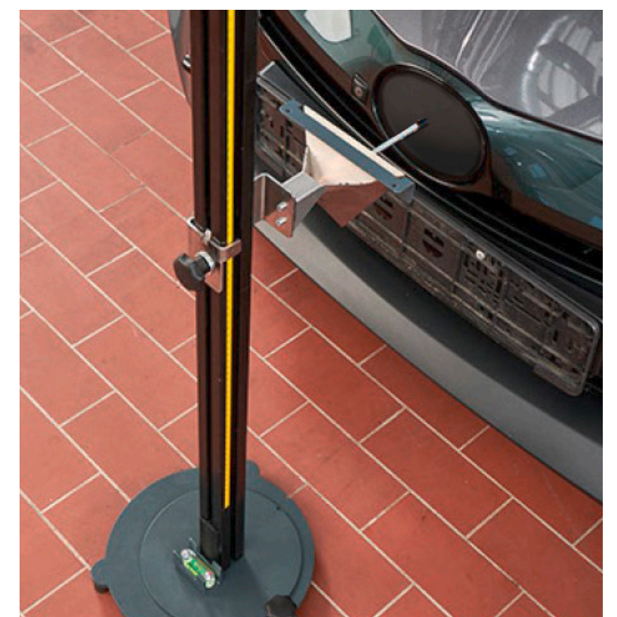
Option to adjust height setting with mechanical indicator pointing on vehicle reference point (emblem)
